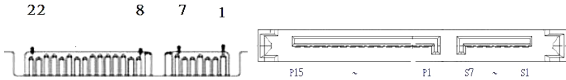
Figure 4: 2.5" SATA SSD Connector Pin Assignment
